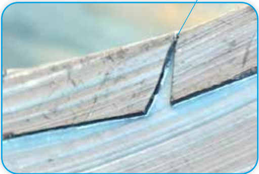
High temperature duct sealant on all spigot to body joints maintains airtightness.
